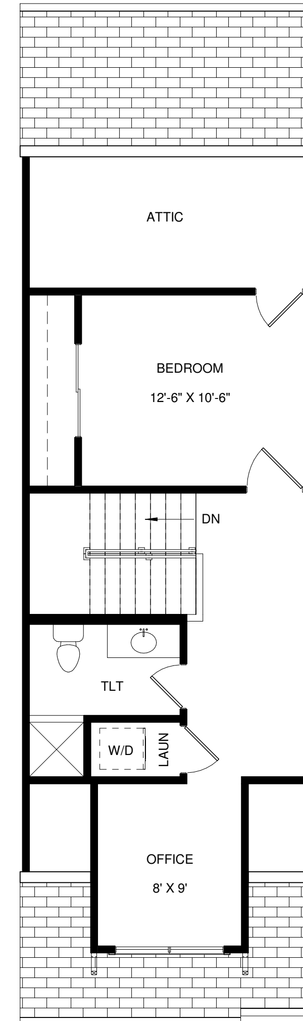
THIRD FLOOR
